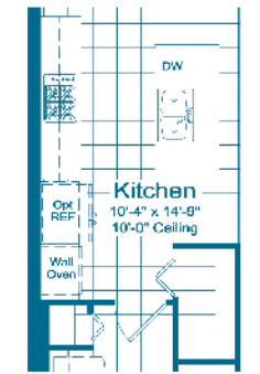
Opt Wall Oven Kitchen
