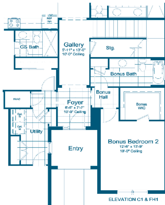
Partial First Floor w/ Opt Bonus Room
